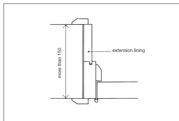
Figure 2 Use of extension lining on thicker partitions
